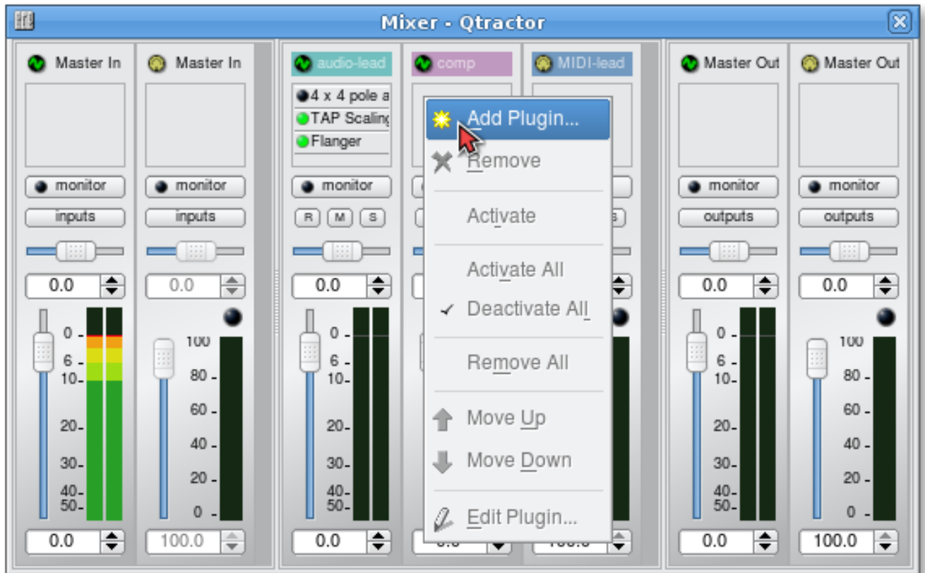
Illustration 3.12: Mixer window showing audio plugin area at top; plugins are added, removed, activated/deactivated, moved in the processing chain and their settings edited using a right-click context menu.
