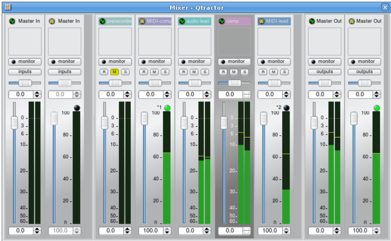
Illustration 3.11: Mixer window
