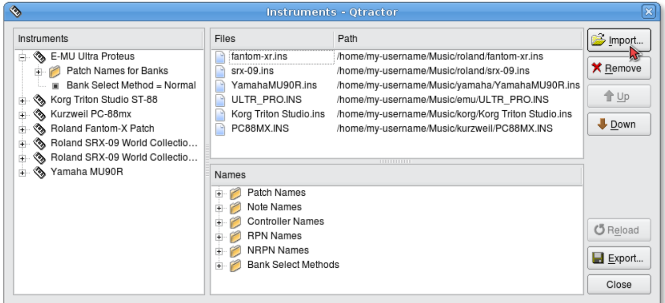
Illustration 3.14: Instruments window, where MIDI instrument definition files, for various popular MIDI tone generators, can be imported, exported and moved.
