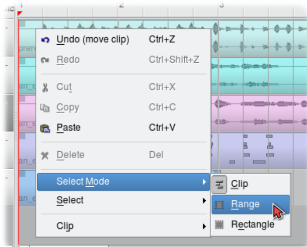
Illustration 3.8: Select Mode context menu (right-click menu)
