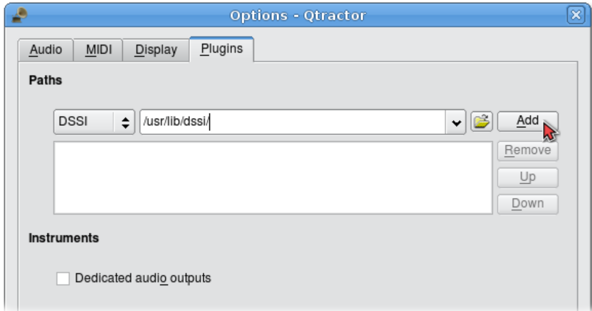
Illustration 3.13: The locations (paths) of LADSPA and DSSI audio plugins can be specified in the View → Options window, under the Plugins tab.
