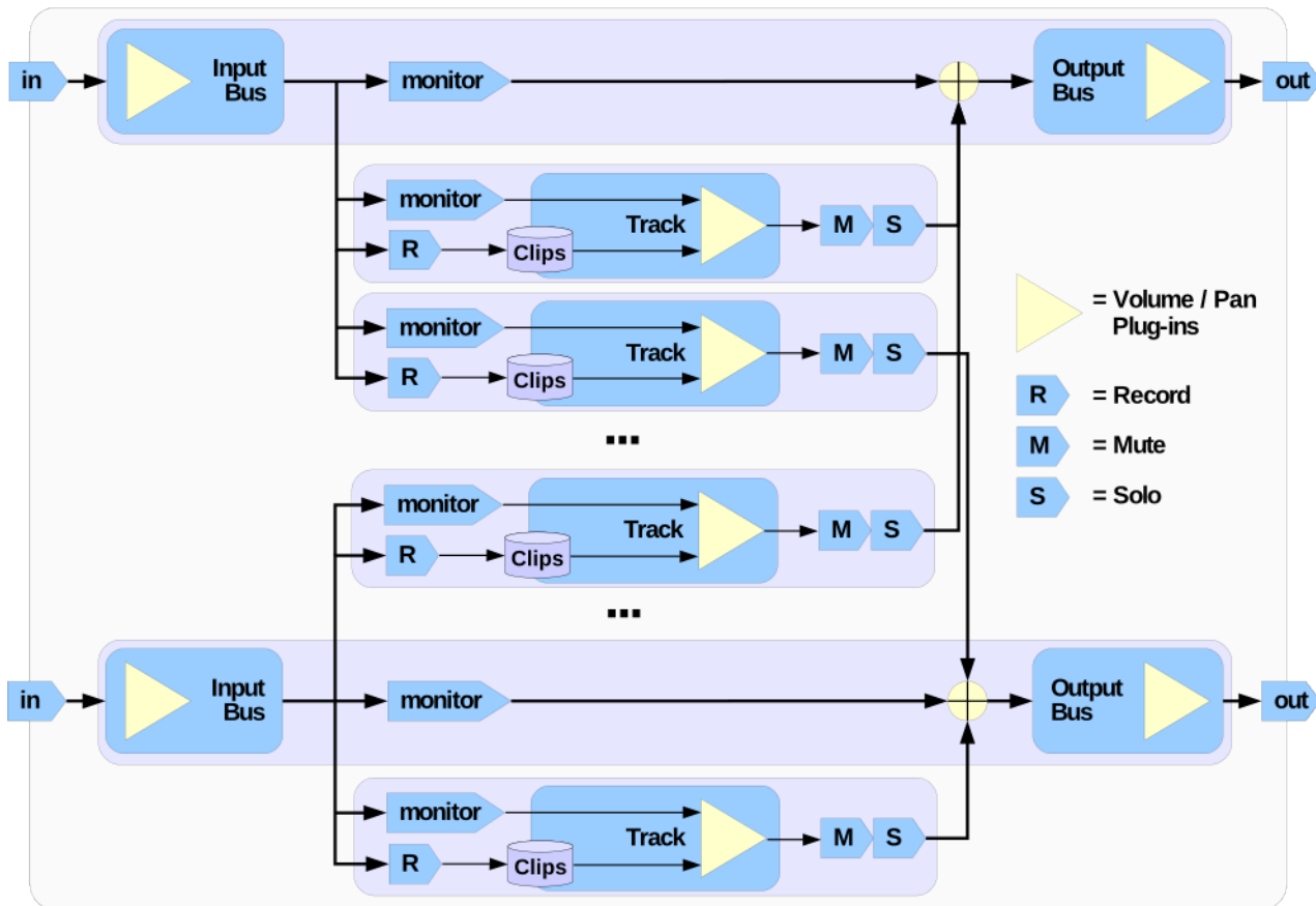
Illustration 3.1: Audio & MIDI data flow, in, through & out of Qtractor
