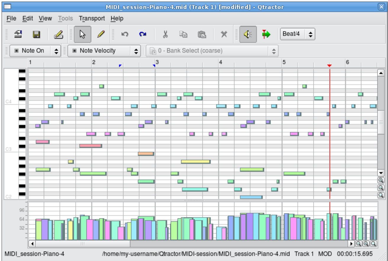
Illustration 3.15: MIDI Editor window, showing notes in a familiar “piano roll” type of graphical display, above, and a graph of their velocities below. The notes and their velocities can be selected and edited in many ways, using the mouse, menu commands and context menus.
